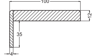
12x100x220 DÜZ PERVAZ
